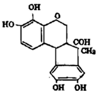
Hematoxylin
