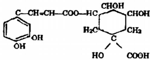
Axit chlorogenic
