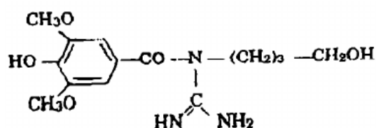
Leonurin
